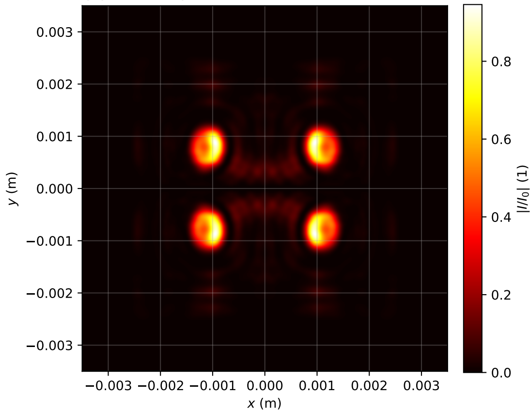
Intensity profile I(x, y, z = 2.627)/I_0 , P_{in}=8.0P_{cr} , artificial time
